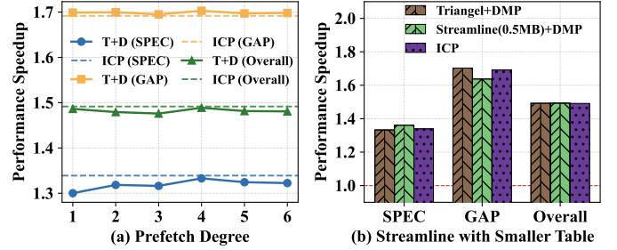
Fig. 16. Sensitivity study for temporal prefetcher degree and table size.
